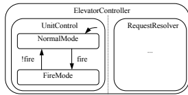
With concurrent RequestResolver
